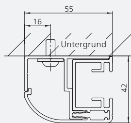
Wandmontage
