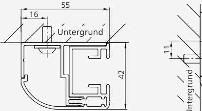
Wandmontage
