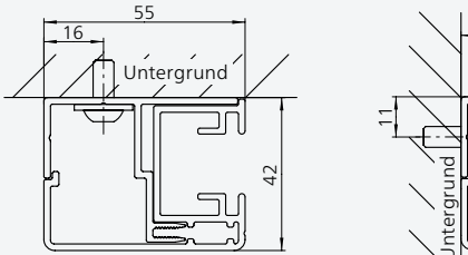
Wandmontage
